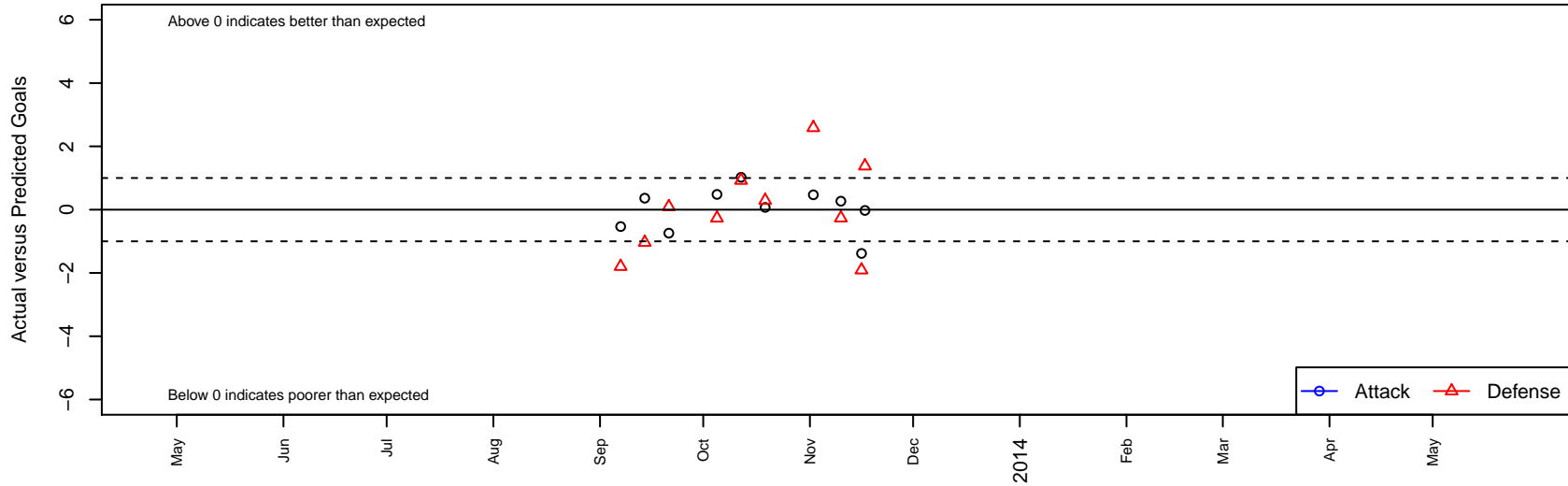
Turlock FC Tornados G00 Dots are actual minus expected GF (blue circles) and GA (red triangles). Blue line is smoothed change in attack strength. Red is smoothed change in defense strength.
